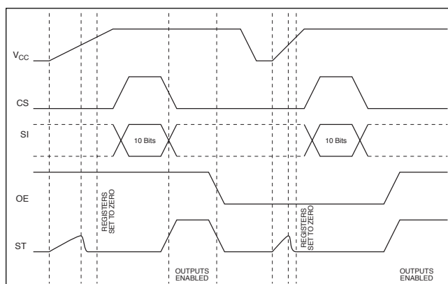
Figure 4. Power-up sequence.
