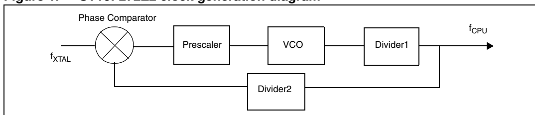
Figure 1. ST10F272Z2 clock generation diagram
