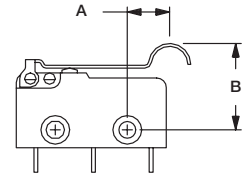
FIG. 5 Simulated Roller
