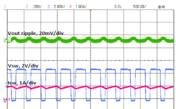
Output Ripple and SW at 1A load V_{in}=5\text{V} / V_{out}=3.3\text{V}
