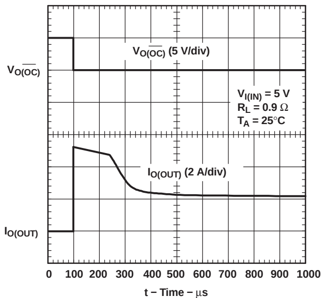
Figure 20. 0.9-Ω Load Connected to an Enabled TPS2023 Device
