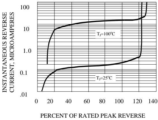
FIG. 3-TYPICAL REVERSE CHARACTERISTICS
