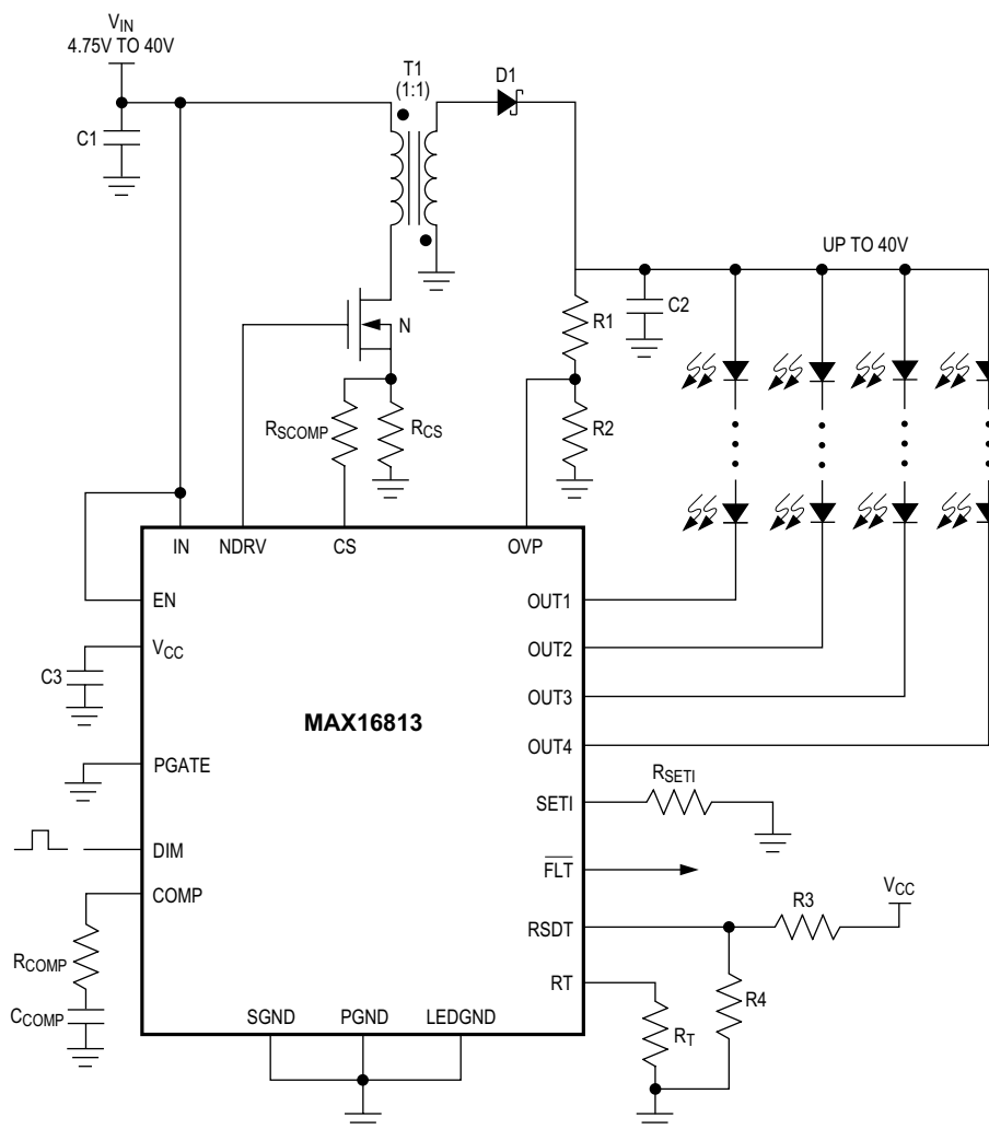
Figure 4. Coupled-Inductor Buck-Boost Configuration
