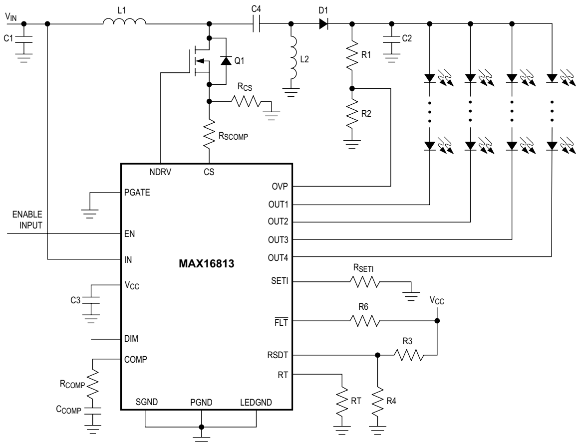
Figure 5. SEPIC LED Driver
