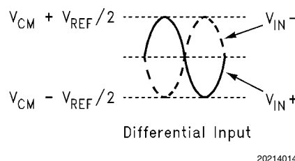
FIGURE 2. Expected Input Signal Range
