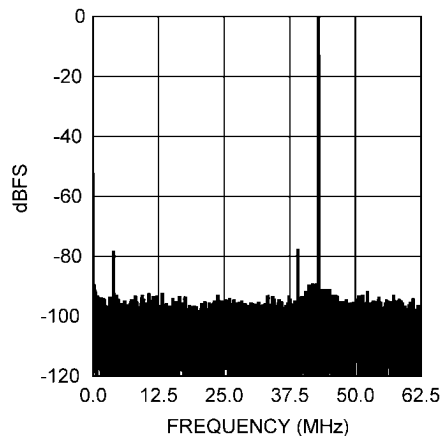
Spectral Response @ 332 MHz Input
