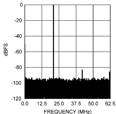
Spectral Response @ 146 MHz Input
