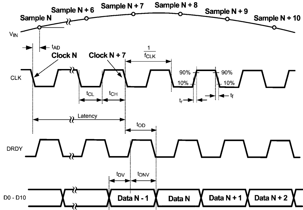
Output Timing
