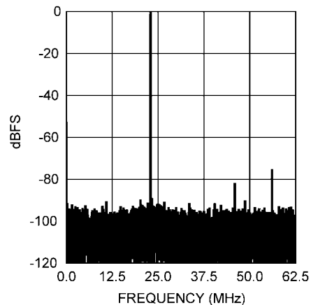
Spectral Response @ 398 MHz Input
