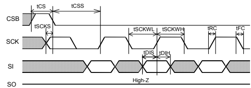
Fig.3 Input timing
