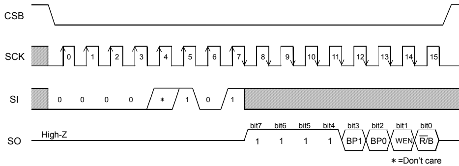
Fig.41 Status register read command (BR25H010/020/040-WC)
