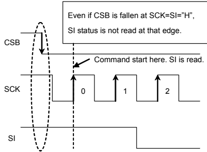
Fig.43 Operating timing
