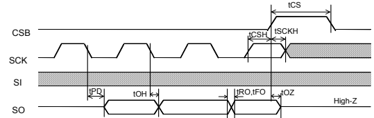
Fig.4 Input / Output timing
