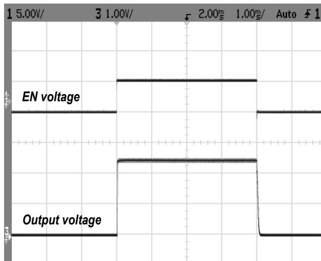
8) Shutdown response
