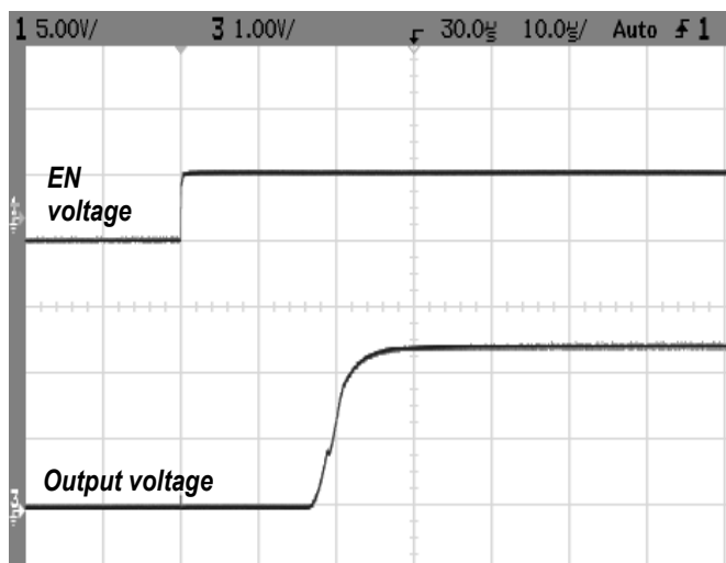
7) Startup response
