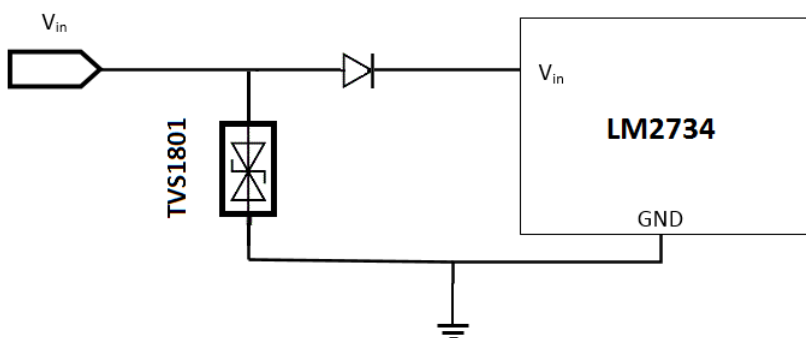
Figure 1. TVS1801 Application Schematic
