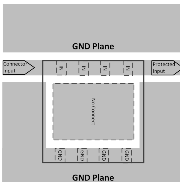
Figure 2. TVS1801 Layout
