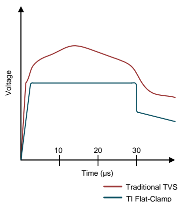
Voltage Clamp Response to 8/20 μs Surge Event
