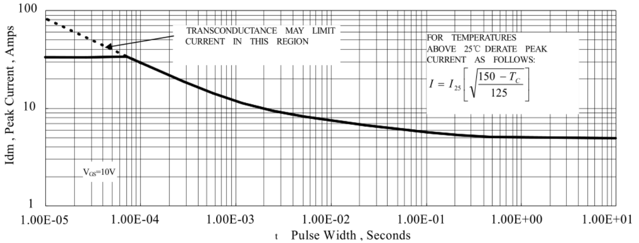
Figure 6 Maximun Peak Current Capability
