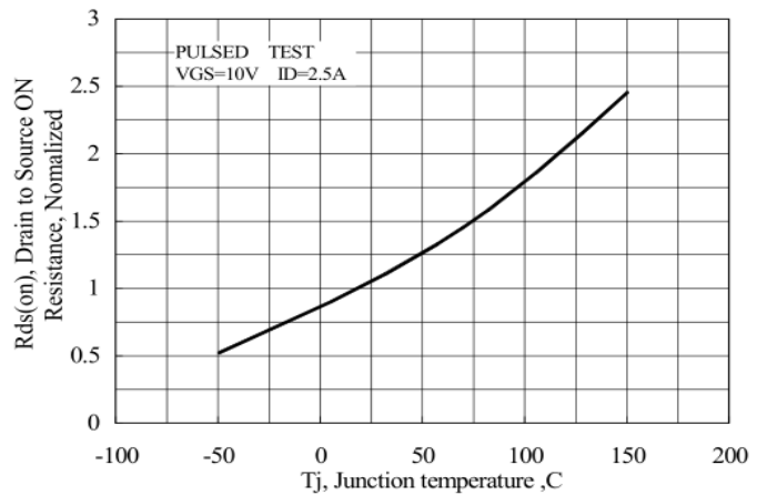
Figure 10 Typical Drian to Source on Resistance vs Junction Temperature
