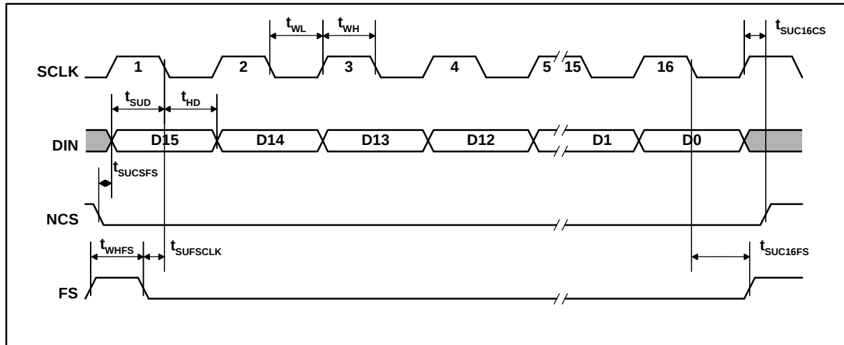
Figure 1 Timing Diagram
