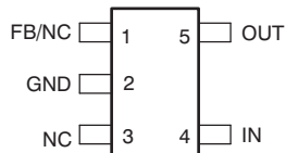
DCK PACKAGE 5-Pin SC70 Top View
