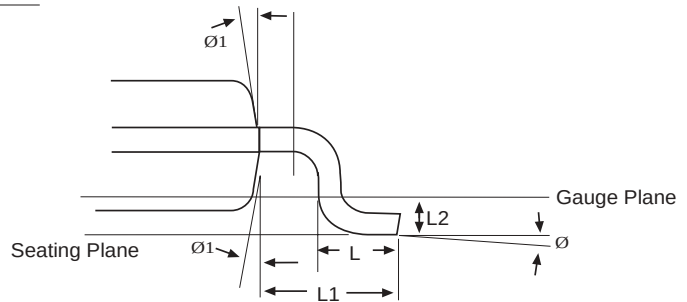
VIEW C
