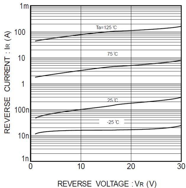
Fig. 2 Reverse characteristics
