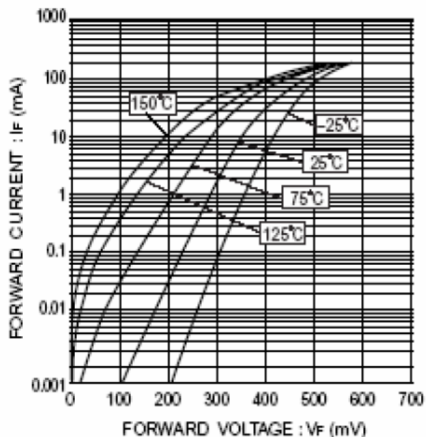
Fig. 1 Forward characteristics
