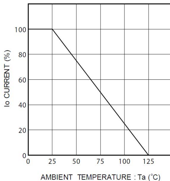
Fig 4. Derating curve (mounting on glass epoxy PCBs)
