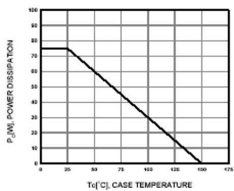
Figure 7. Power Derating
