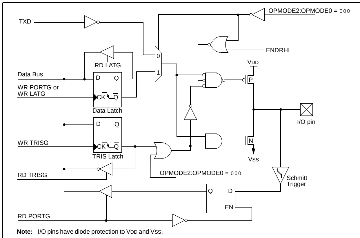
FIGURE 10-16: RG0/CANTX1 PIN BLOCK DIAGRAM
