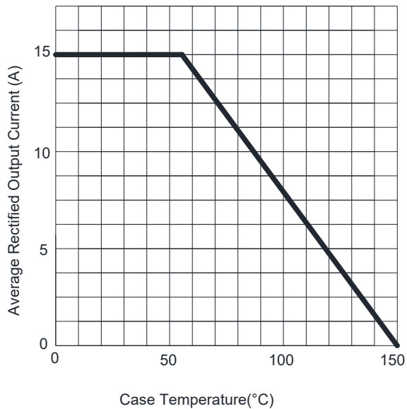
FIG1:Io-Tc Curve
