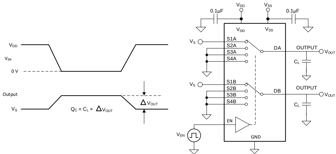
图 24. Charge-Injection Measurement Setup
