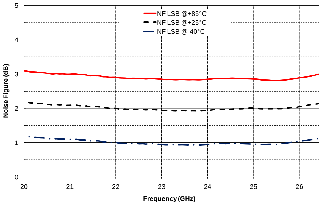
Noise Figure in supradyn mode versus frequency
