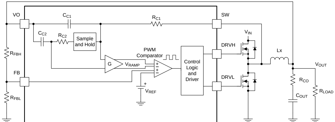
Figure 40. D-CAP3 Mode
