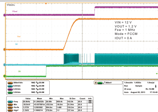
Figure 22. Start-Up
