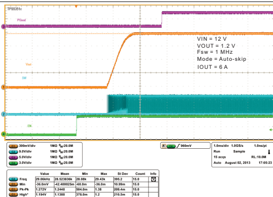
Figure 23. Start-Up
