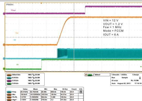
Figure 24. Start-Up
