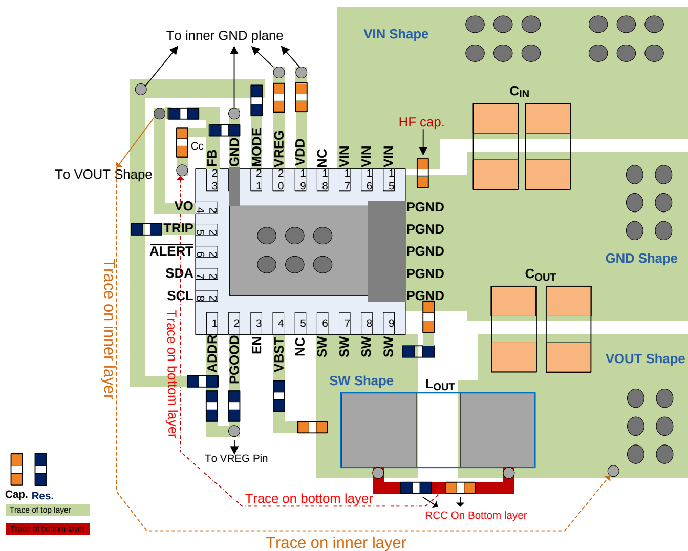
Figure 65. Layout Recommendation
