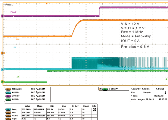
Figure 29. Pre-Bias Operation
