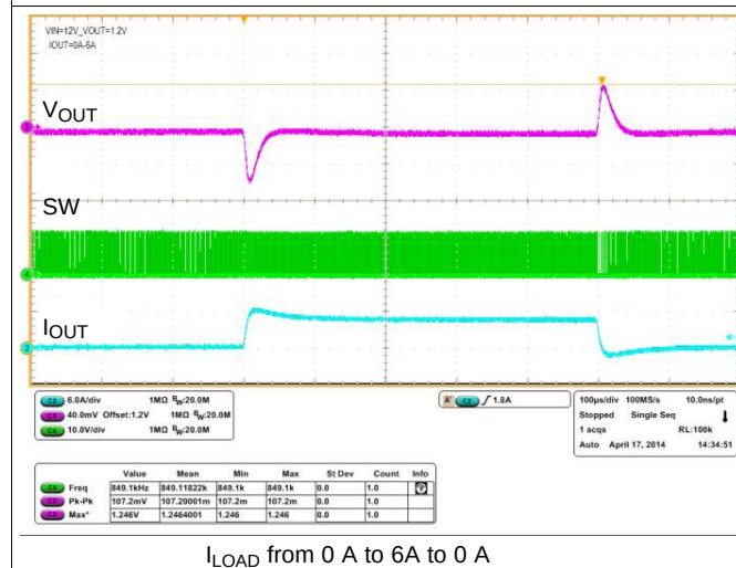
Figure 61. Full Cycle Load Transient
