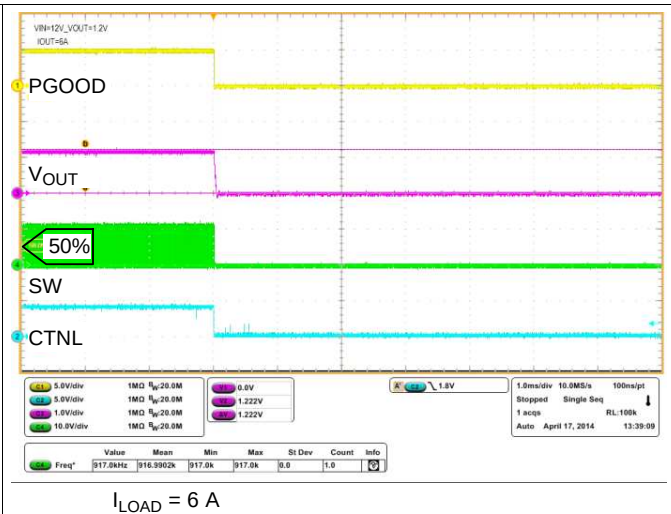
Figure 58. Shutdown Sequence
