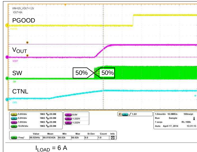
Figure 57. Start-Up Sequence
