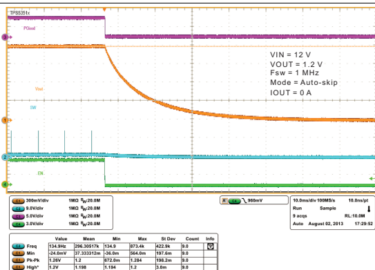
Figure 25. Shutdown Operation
