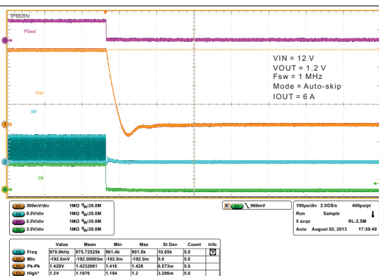
Figure 27. Shutdown Operation
