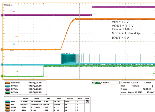
Figure 21. Start-Up
