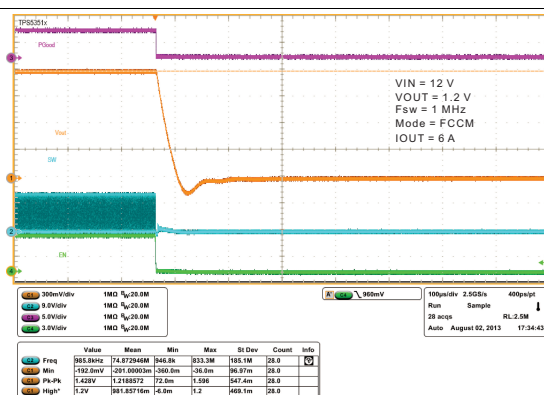
Figure 28. Shutdown Operation
