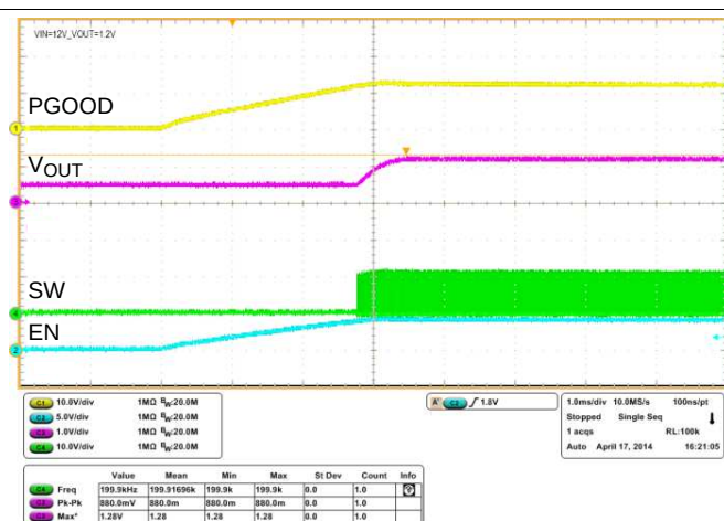
Figure 64. Pre-Bias Start-Up
