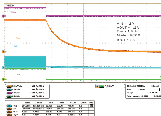
Figure 26. Shutdown Operation
