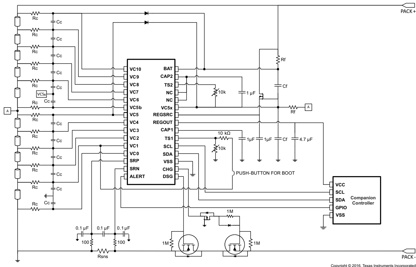
图 9-2. BQ76930 With BQ78350 Companion Controller IC
