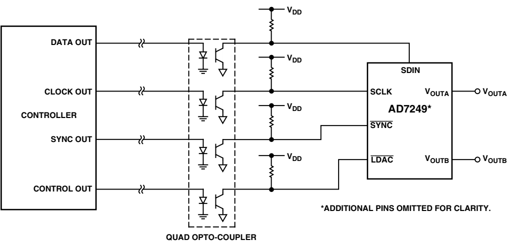
Figure 16. Opto-Isolated Interface
