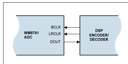
Figure 6 Slave Mode
