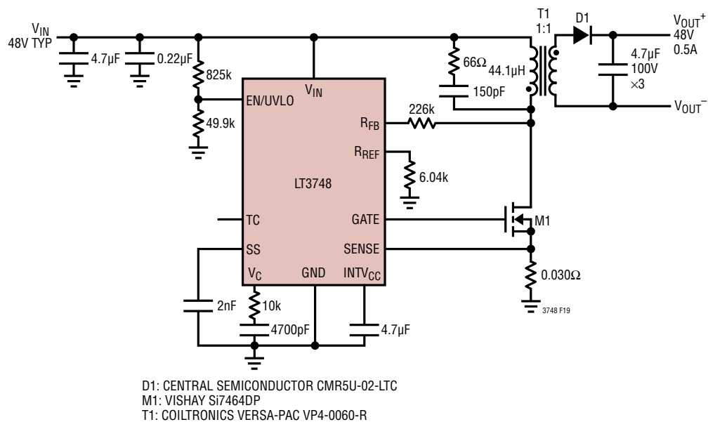
Figure 19. 48V, 0.5A Supply from 24V to 96V Input
