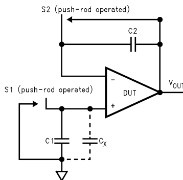
Figure 25. Simple Input Bias Current Test Circuit
