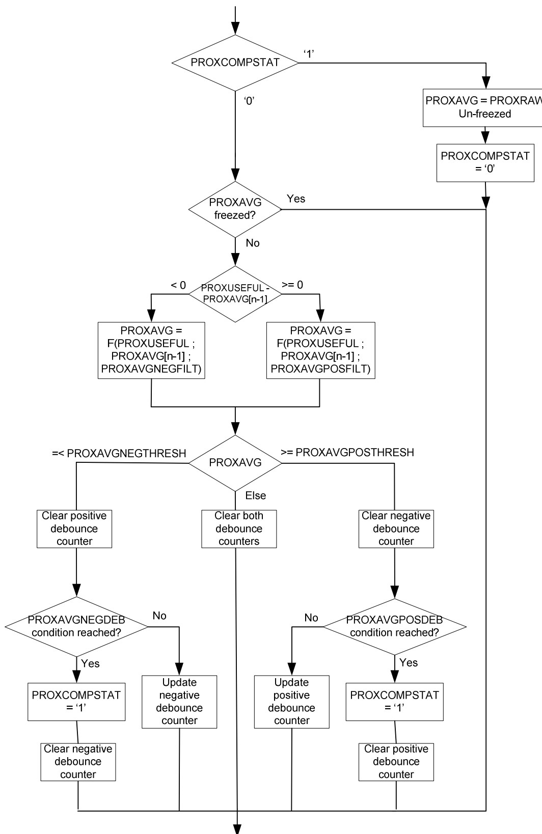
Figure 36 – ProxAvg Update
