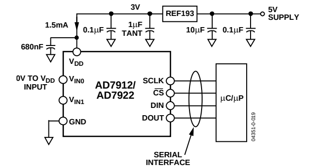
Figure 22. REF193 as Power Supply to AD7912/AD7922
