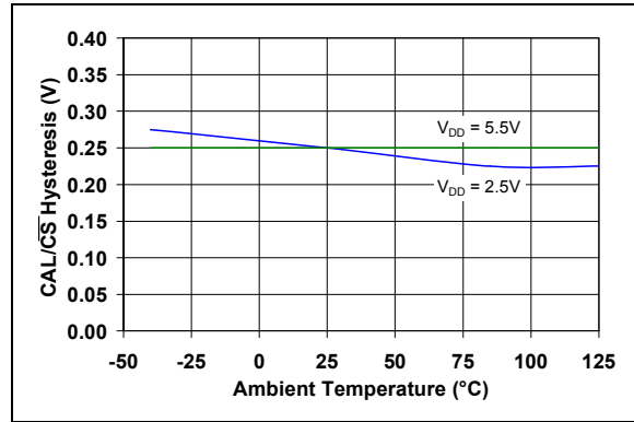
FIGURE 2-47: \text{CAL/CS} Hysteresis vs. Ambient Temperature.
