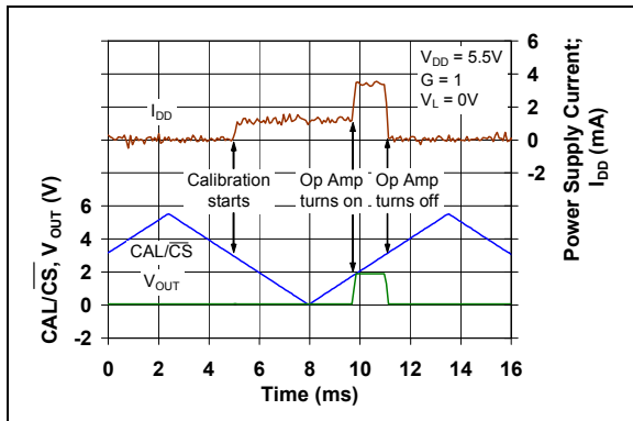
FIGURE 2-46: \text{CAL/CS} Voltage, Output Voltage and Supply Current (for Side A) vs. Time with V_{DD} = 5.5\text{V} .
