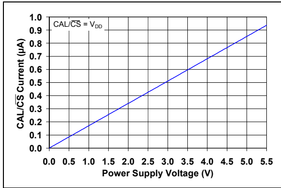
FIGURE 2-44: \text{CAL/CS} Current vs. Power Supply Voltage.
