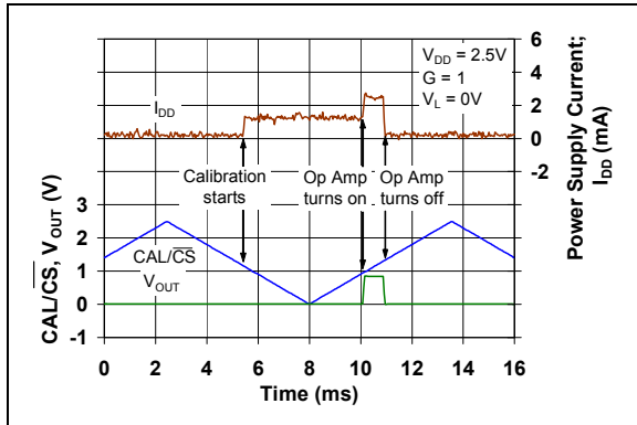
FIGURE 2-45: \text{CAL/CS} Voltage, Output Voltage and Supply Current (for Side A) vs. Time with V_{DD} = 2.5\text{V} .
