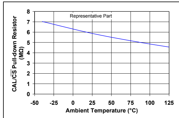
FIGURE 2-49: \text{CAL/CS} 's Pull-Down Resistor ( R_{PD} ) vs. Ambient Temperature.
