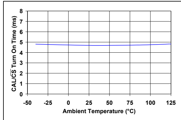
FIGURE 2-48: \text{CAL/CS} Turn-On Time vs. Ambient Temperature.
