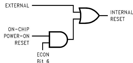
Figure 17. Reset Logic
