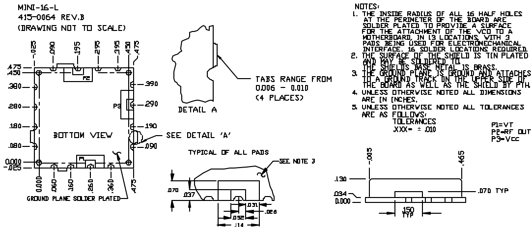
PHYSICAL DIMENSIONS
