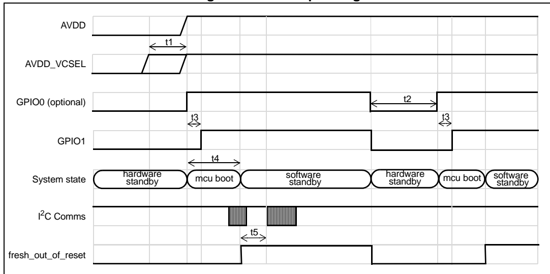
Figure 9. Power-up timing
