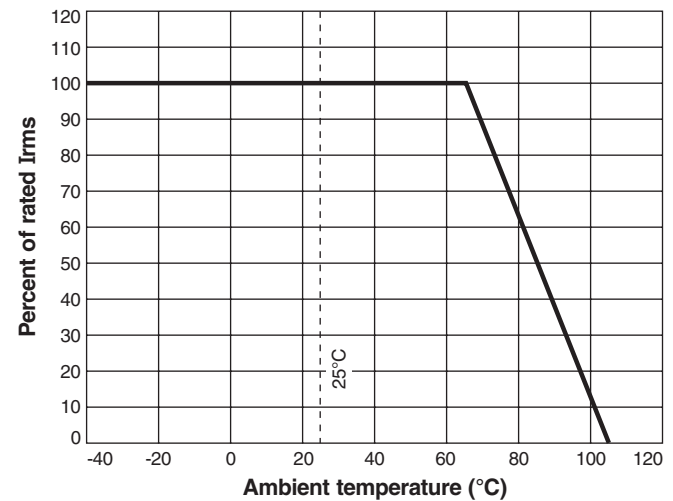
Irms Derating
