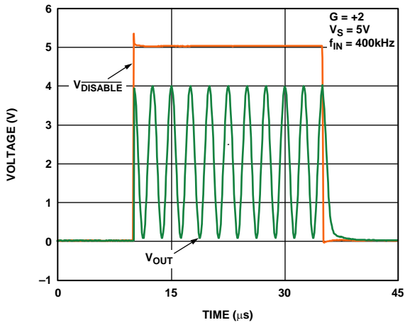
Figure 23. Enable/Disable Time
