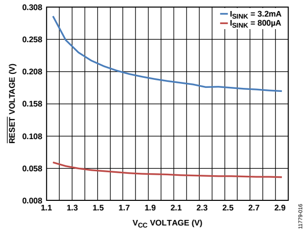
Figure 16. \overline{\text{RESET}} Open-Drain V_{OL} Voltage vs. V_{CC} Voltage ( V_{TH} = 3\text{ V} )
