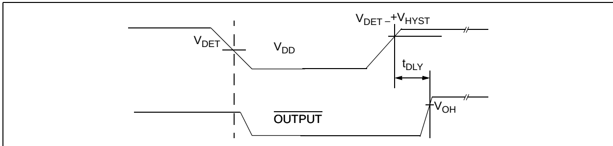
FIGURE 1-1: Timing Diagram.
