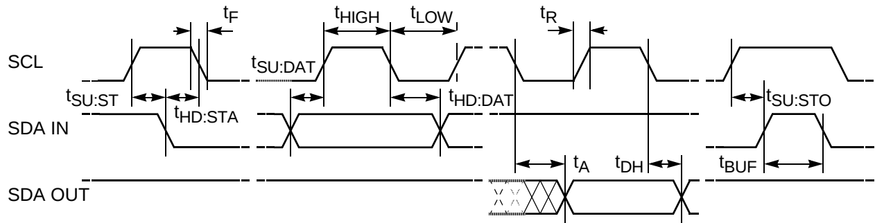
Figure 22. Bus Timing
