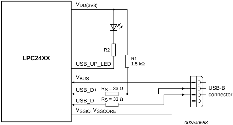
Fig 22. LPC2478 USB interface on a bus-powered device
