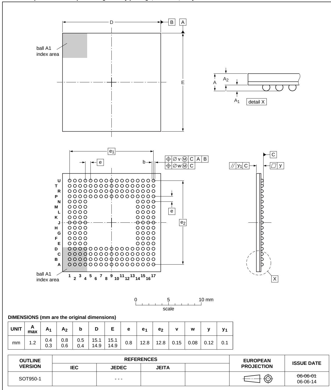
TFBGA208: plastic thin fine-pitch ball grid array package; 208 balls; body 15 x 15 x 0.7 mm
