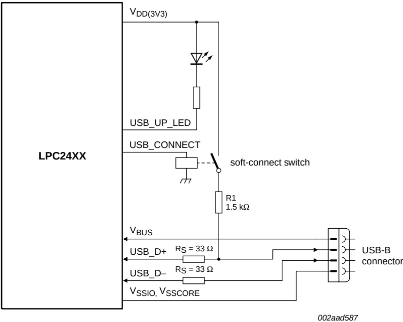
Fig 21. LPC2478 USB interface on a self-powered device
