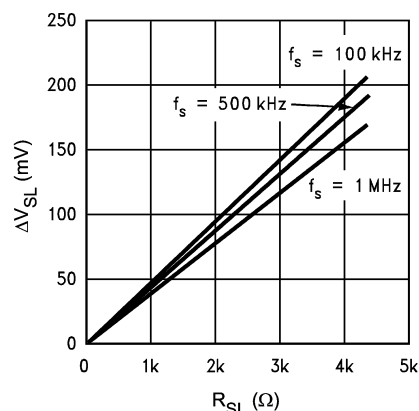
Figure 28. External Slope Compensation \Delta V_{SL} vs R_{SL}
