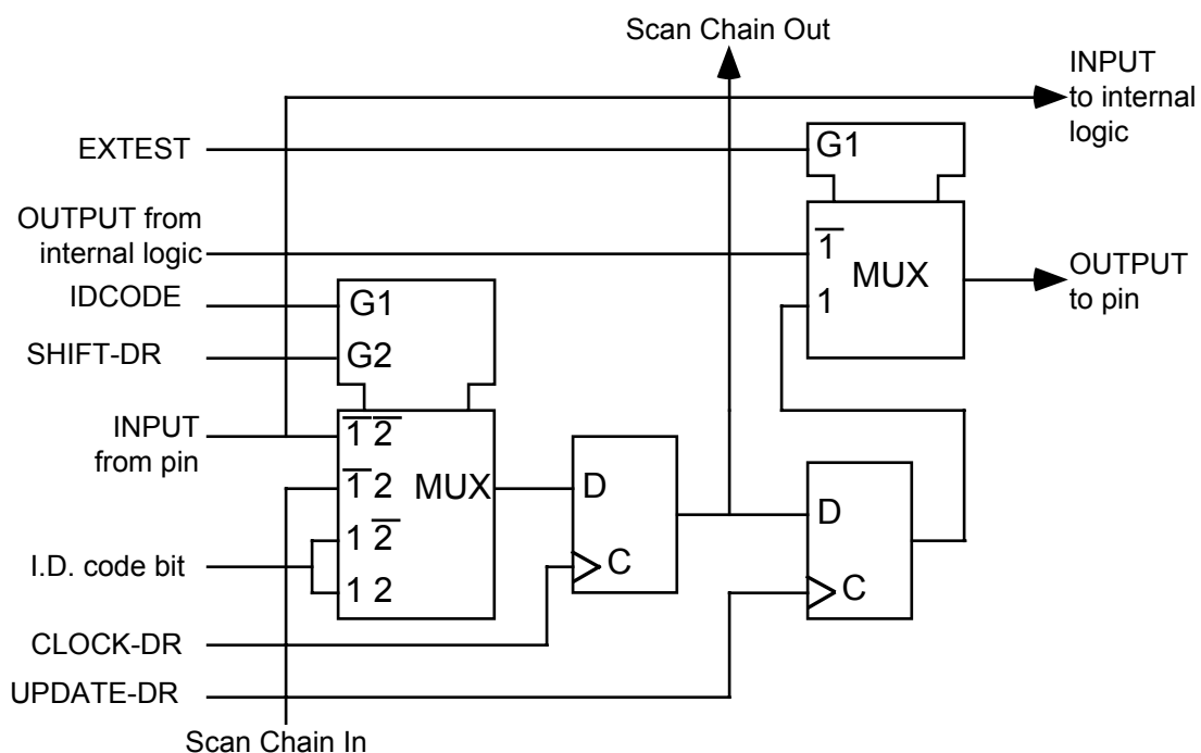
Figure 7 – Bi-directional Cell (IO_CELL)
