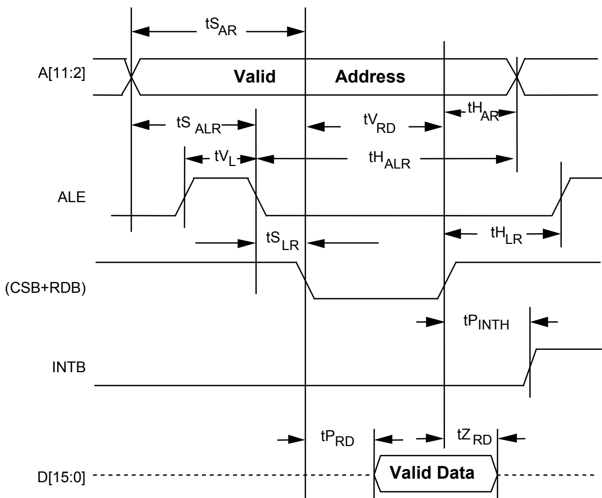
Figure 31 – Microprocessor Read Access Timing
