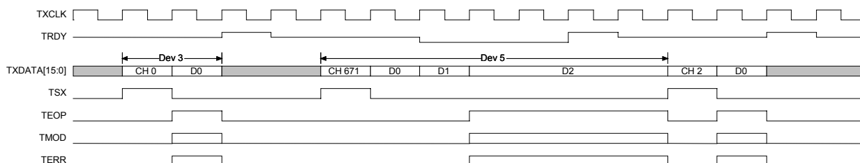
Figure 21 – Transmit APPI Timing (Special Conditions)
