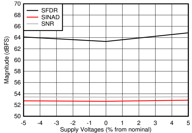
F_{IN} = 347 MHz
