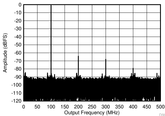
Figure 7-11. Single Tone FFT at 99.997 MHz and -1 dBFS F_S = 1000\text{MSPS} , Low Power Mode
