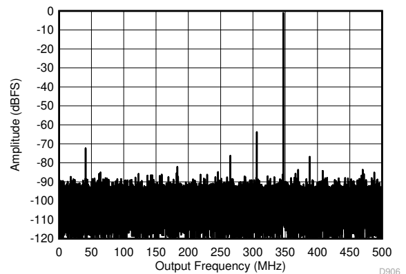
Figure 7-12. Single Tone FFT at 347 MHz and -1 dBFS F_S = 1000\text{MSPS} , Low Power Mode
