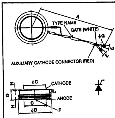
FT1500DV Outline Drawing
