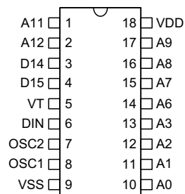
HT692 – 18 DIP
