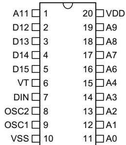
HT614 – 20 DIP/SOP
