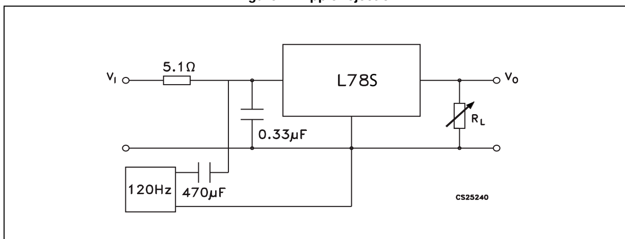
Figure 7. Ripple rejection
