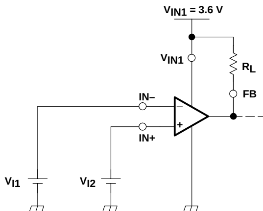
Figure 5. V_{OL}
