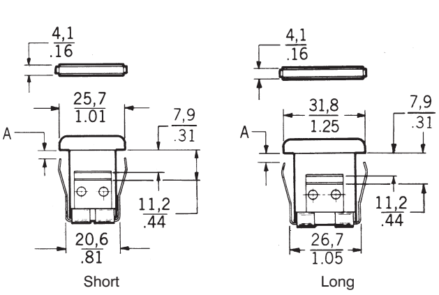
Mounting barriers
