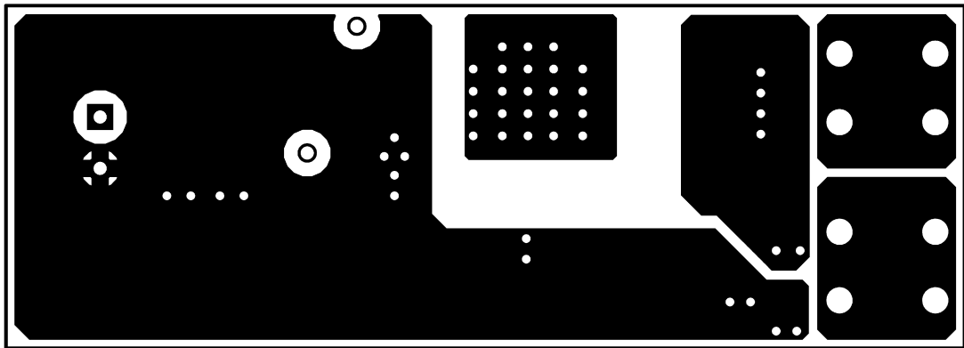
Figure 23. Solder Side
