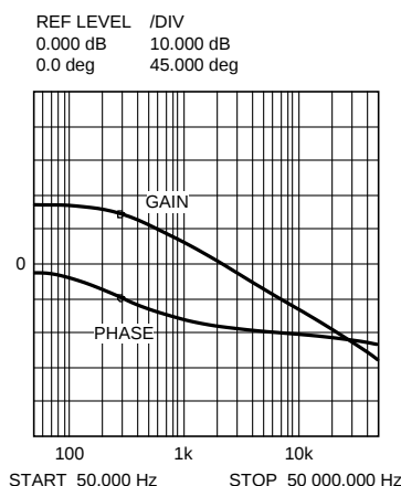
Figure 17. Gain and Phase of Modulator R LOAD = 5 Ohms and C OUT = 177μF
