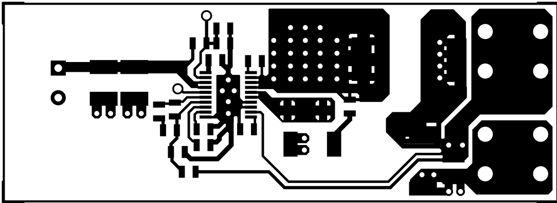
Figure 22. Component Side
