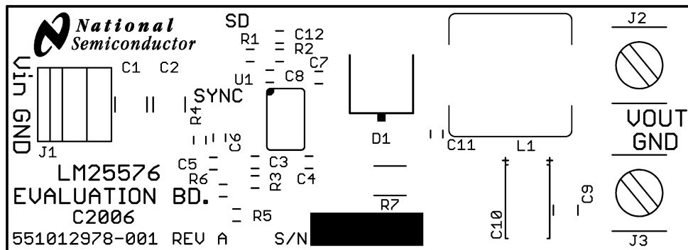
Figure 24. Silkscreen
