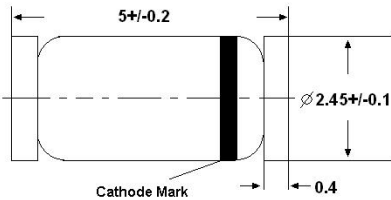
Glass case MELF Dimensions in mm
