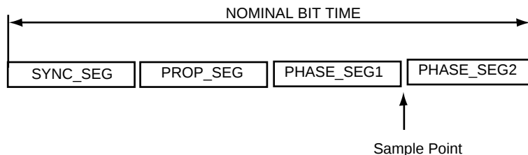
Figure 38-4. Partition of the CAN Bit Time
